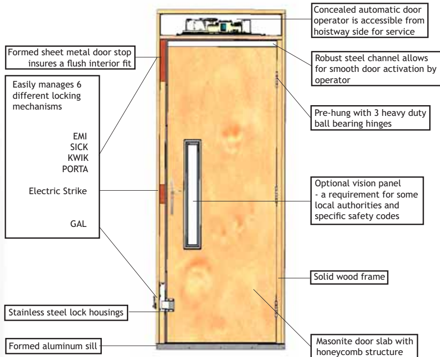
FLUSH MOUNTED DOOR INSIDE HOISTWAY
